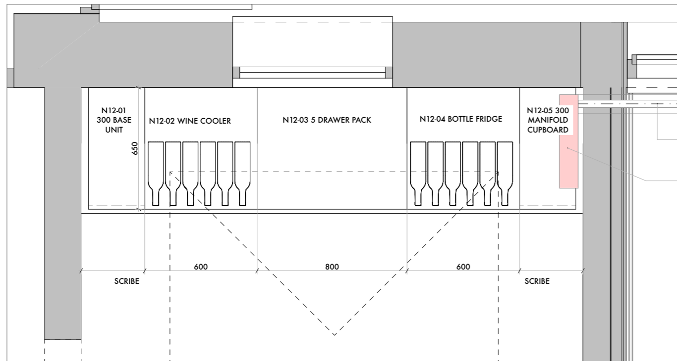
BAR FITTINGS
