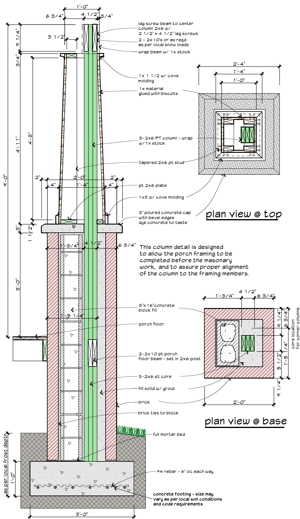
F6 Porch Detail scale 1" = 1'-0"
